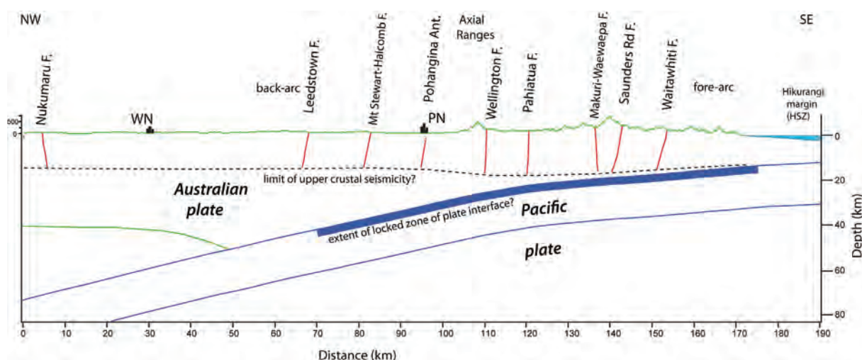
Figure 2.1 Simplified tectonic cross-section of the Horizons Region from offshore of Akitio in the east to near Whanganui (WN). The cross-section intercepts several well-known active upper crustal faults and includes the Hikurangi subduction zone (HSZ). The location of Palmerston North (PN) is also indicated. Ant, anticline; F, fault.
