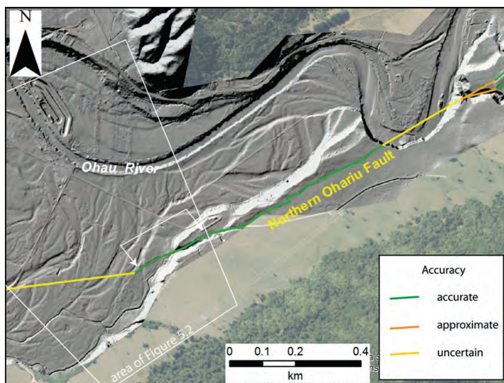
Figure 5.3 A) LiDAR hill-shade image (with a colour orthophoto underlay) of the Ohau River area showing the Northern Ohariu Fault. B) Annotated version of the same image. The area of the photograph in Figure 5.2 is shown, and the double arrow shows the part of the fault shown in Figure 5.2, which is accurately located.
