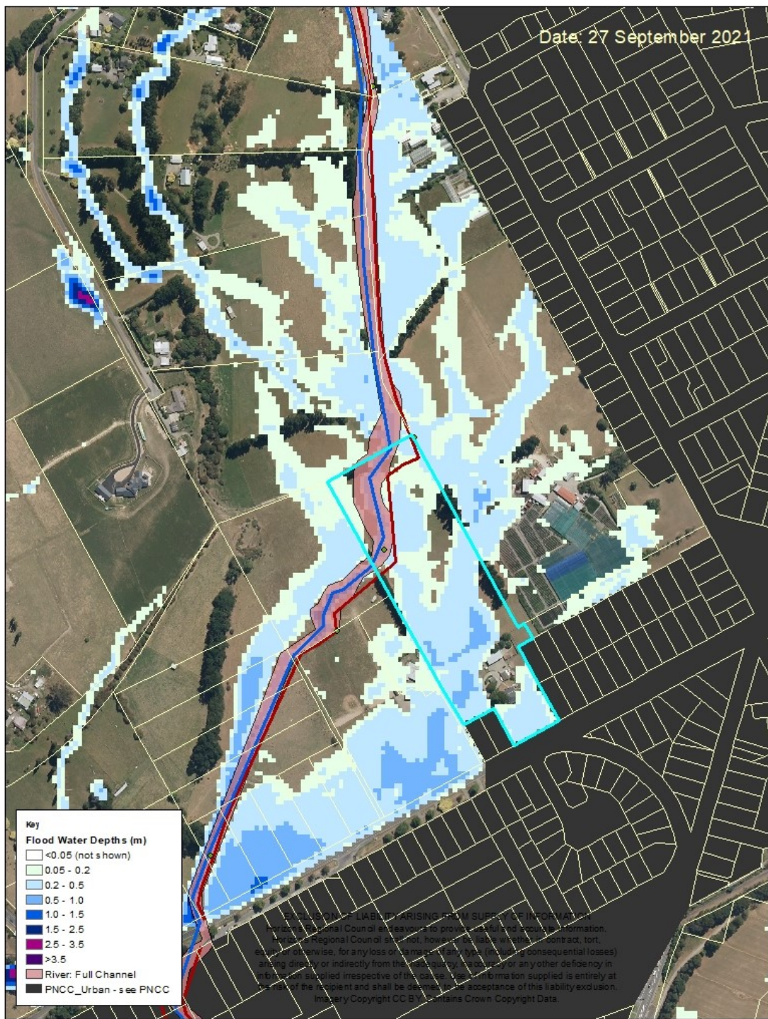
0.5% AEP (1 in 200 year) Modelled Flood Depths for 94 Mulgrave Street, Ashhurst
