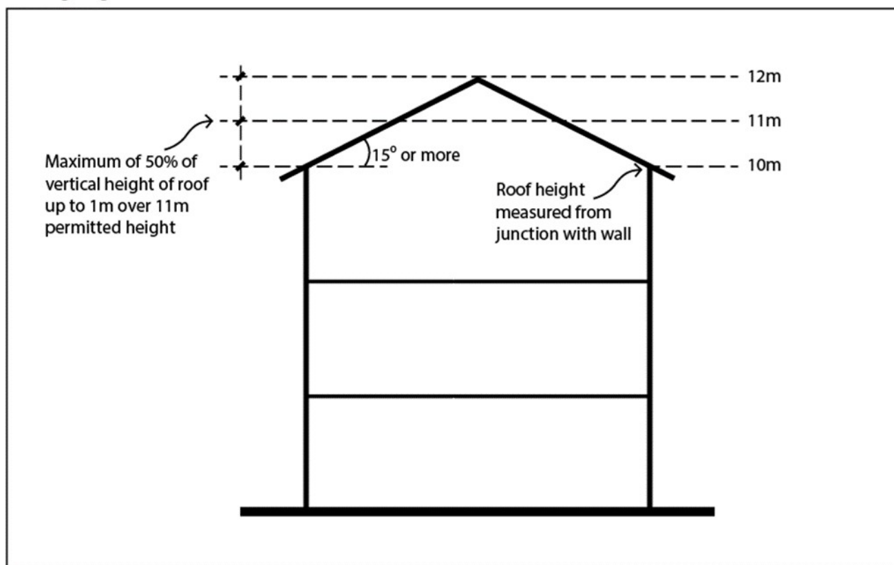
Figure 11.5B Building Height
